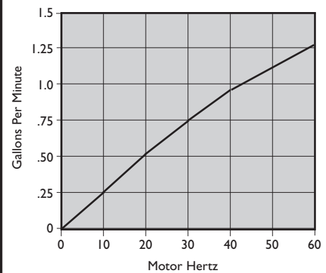
ELECTRIC PM ANCHOR PUMP® 101E FLOW PERFORMANCE
