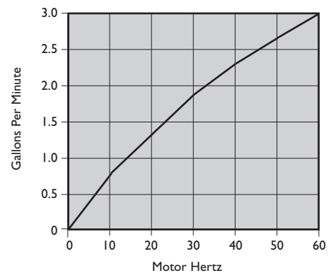
ELECTRIC PM ANCHOR PUMP® 102E FLOW PERFORMANCE
