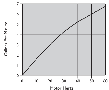
ELECTRIC PM ANCHOR PUMP® 103E FLOW PERFORMANCE
